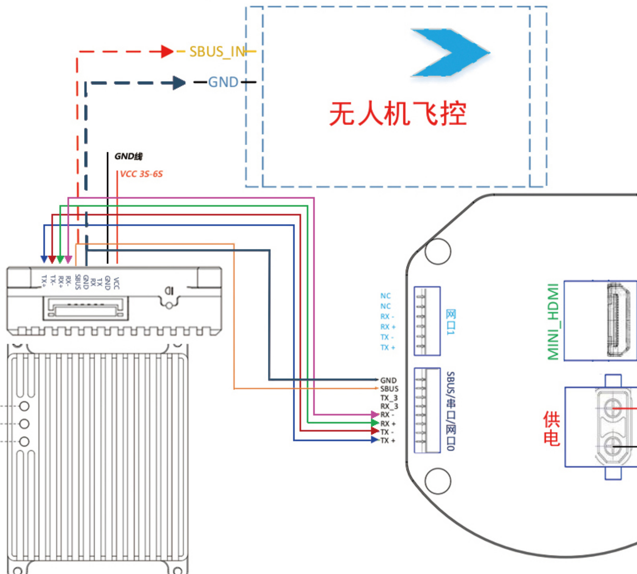
K11与TOPOTEK-(6P+8P)云台相机对接示意图
