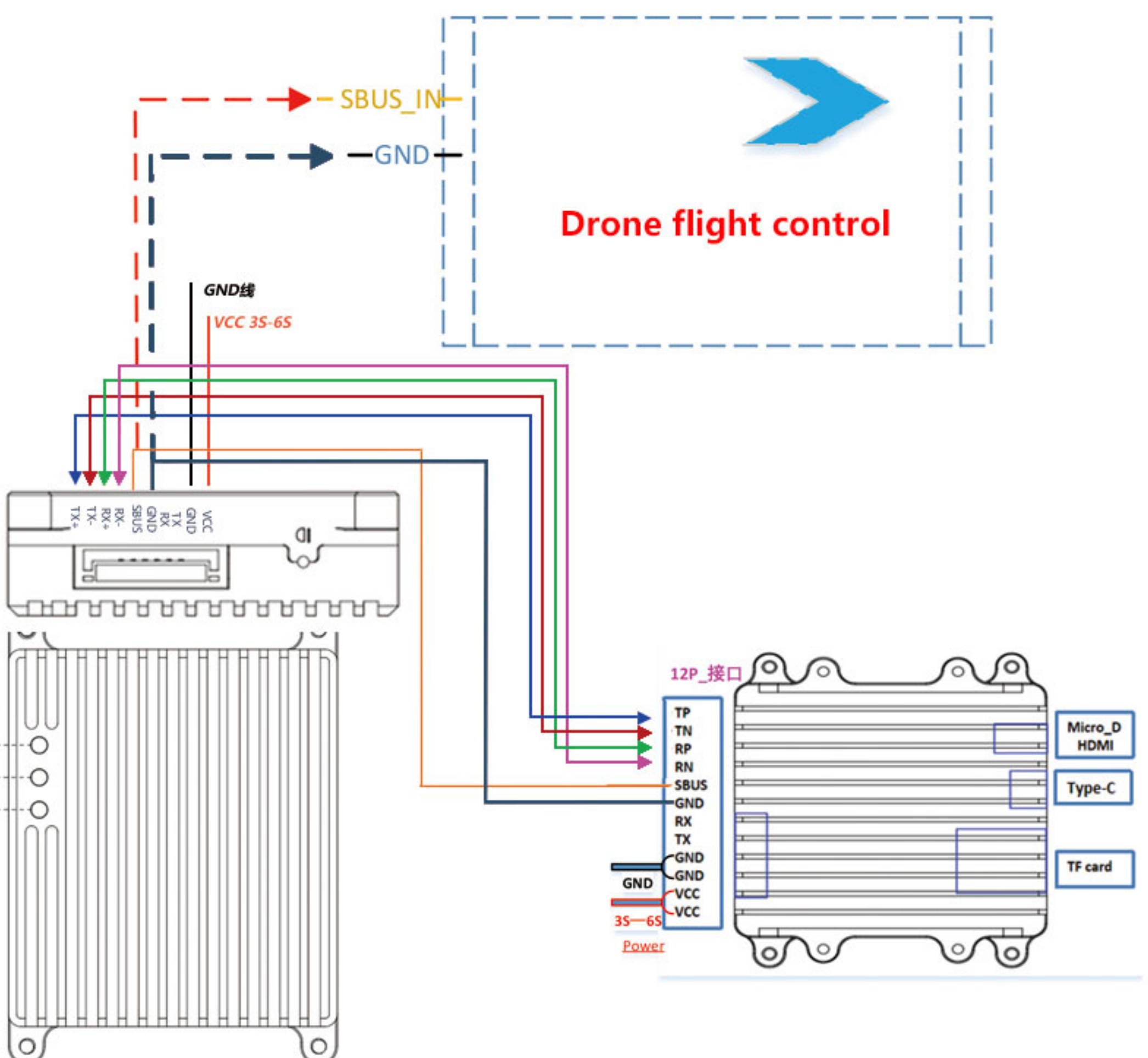
K11andTOPOTEK-12PSchematic diagram of gimbal-camera docking
