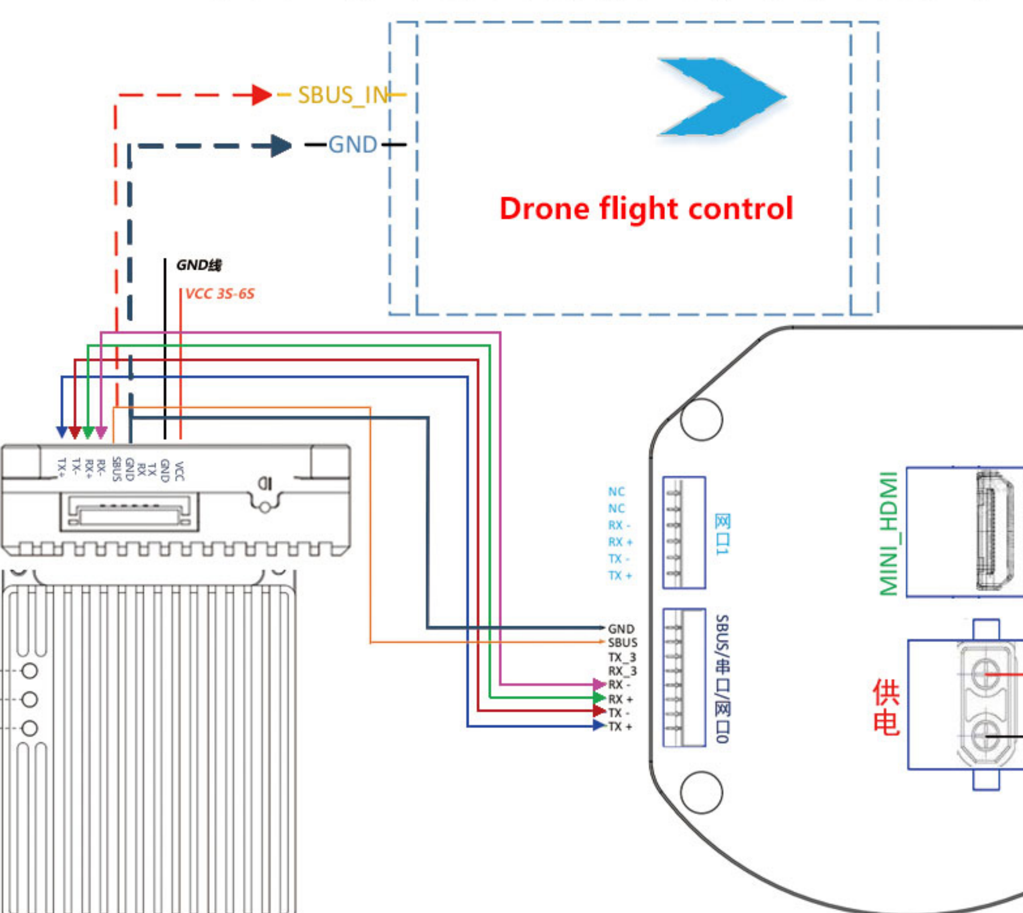
K11与TOPOTEK-(6P+8P)Schematic diagram of gimbal-camera docking
