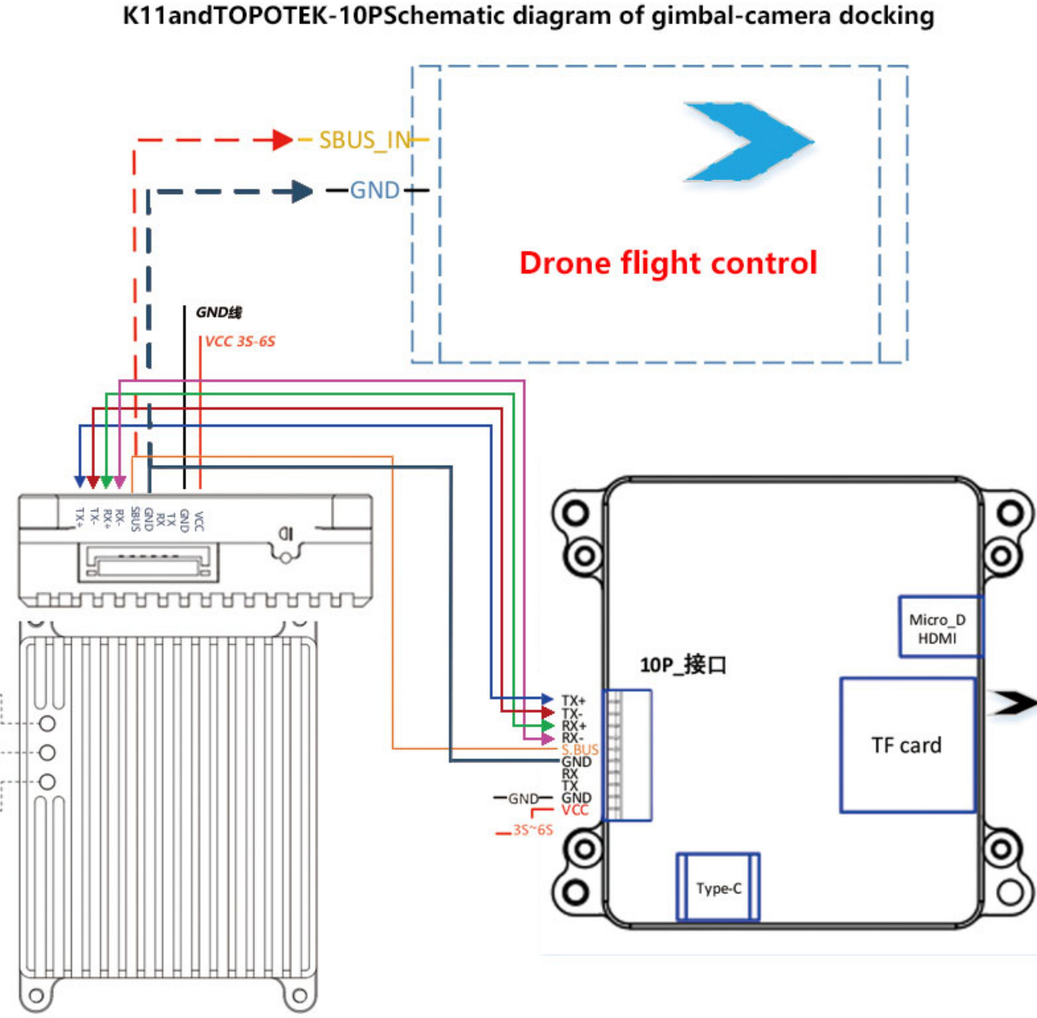
K11andTOPOTEK-10PSchematic diagram of gimbal-camera docking
